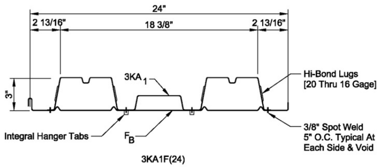
FIGURE 1—CELLULAR DECK DETAILS
